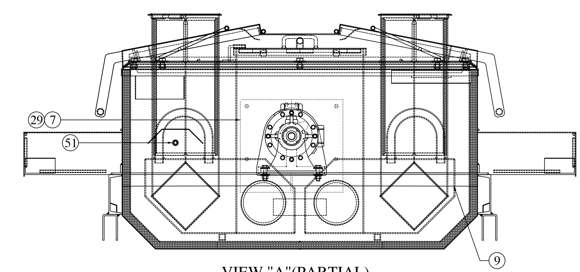
VIEW "A"(PARTIAL)
