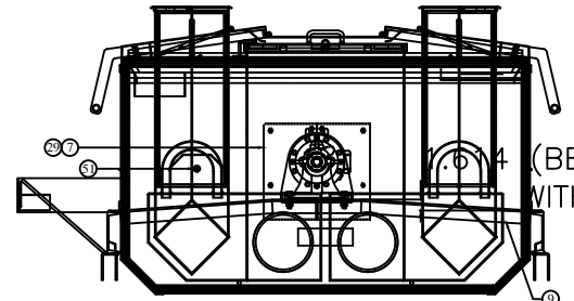
VIEW "A"(PARTIAL)
